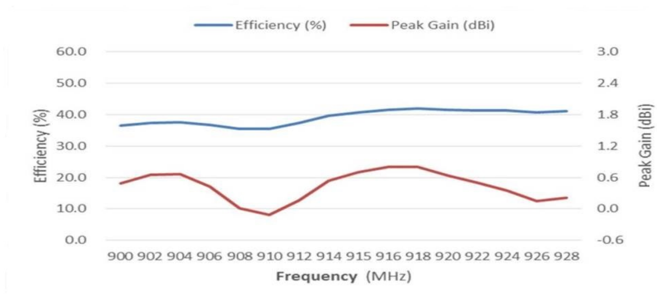
Figure 3: Efficiency vs. Frequency chart
