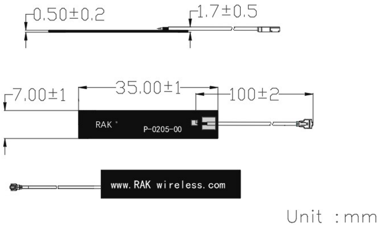
Figure 4: Antenna dimensions
