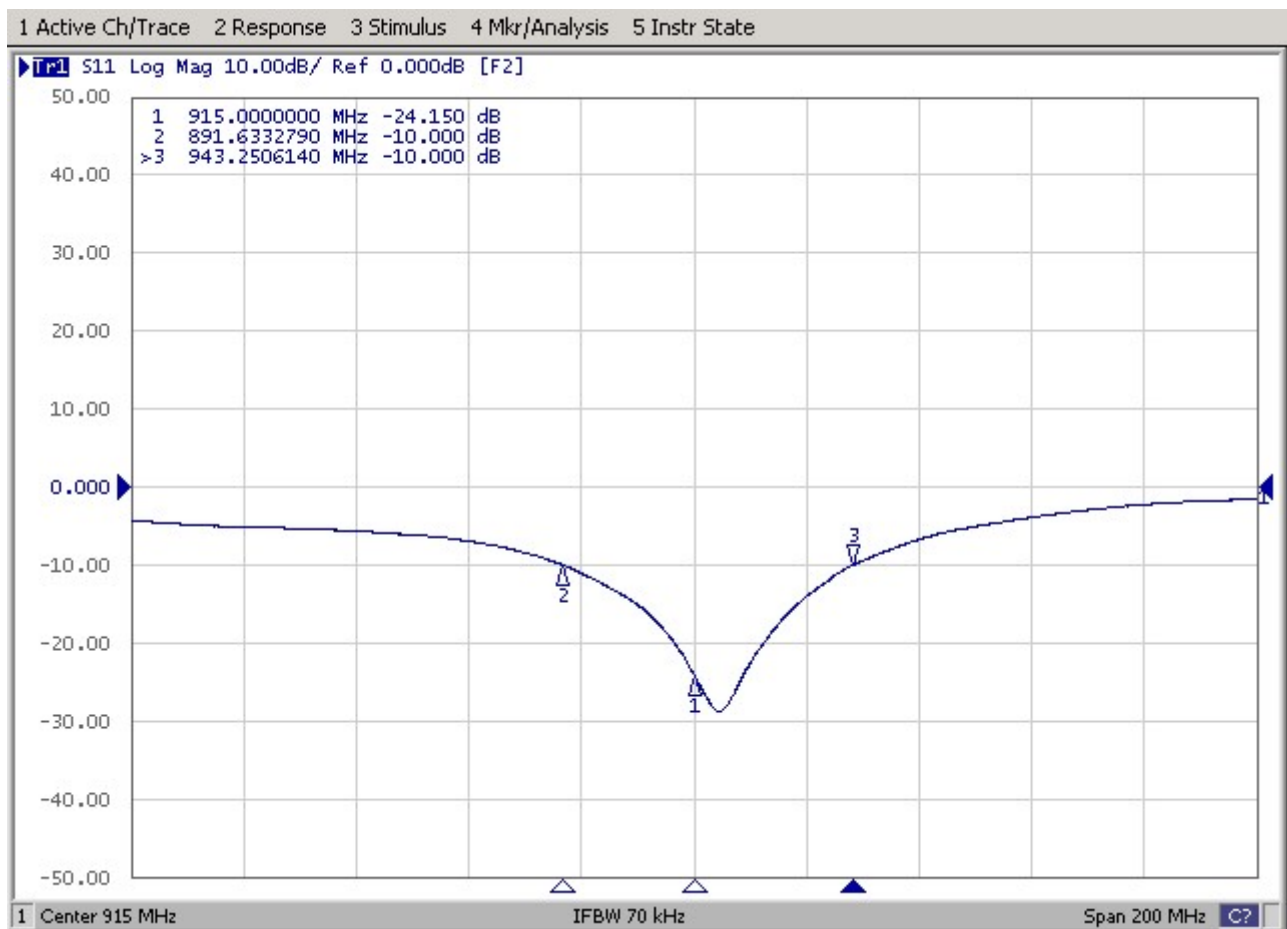
Figure 1: Return loss
