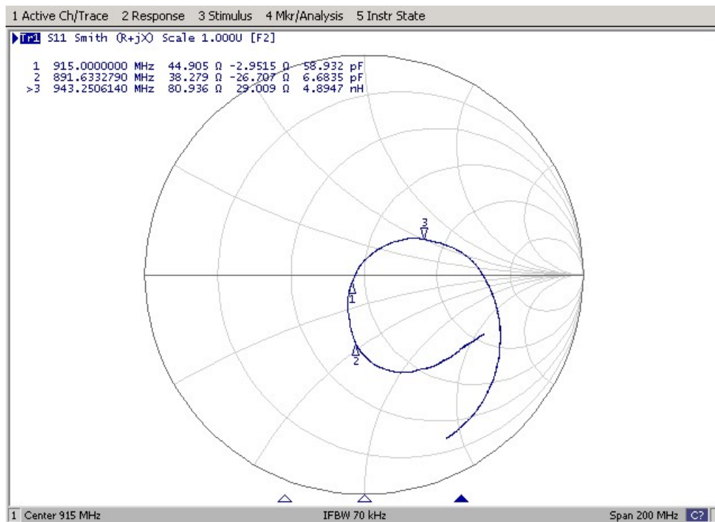
Figure 2: Smith chart
